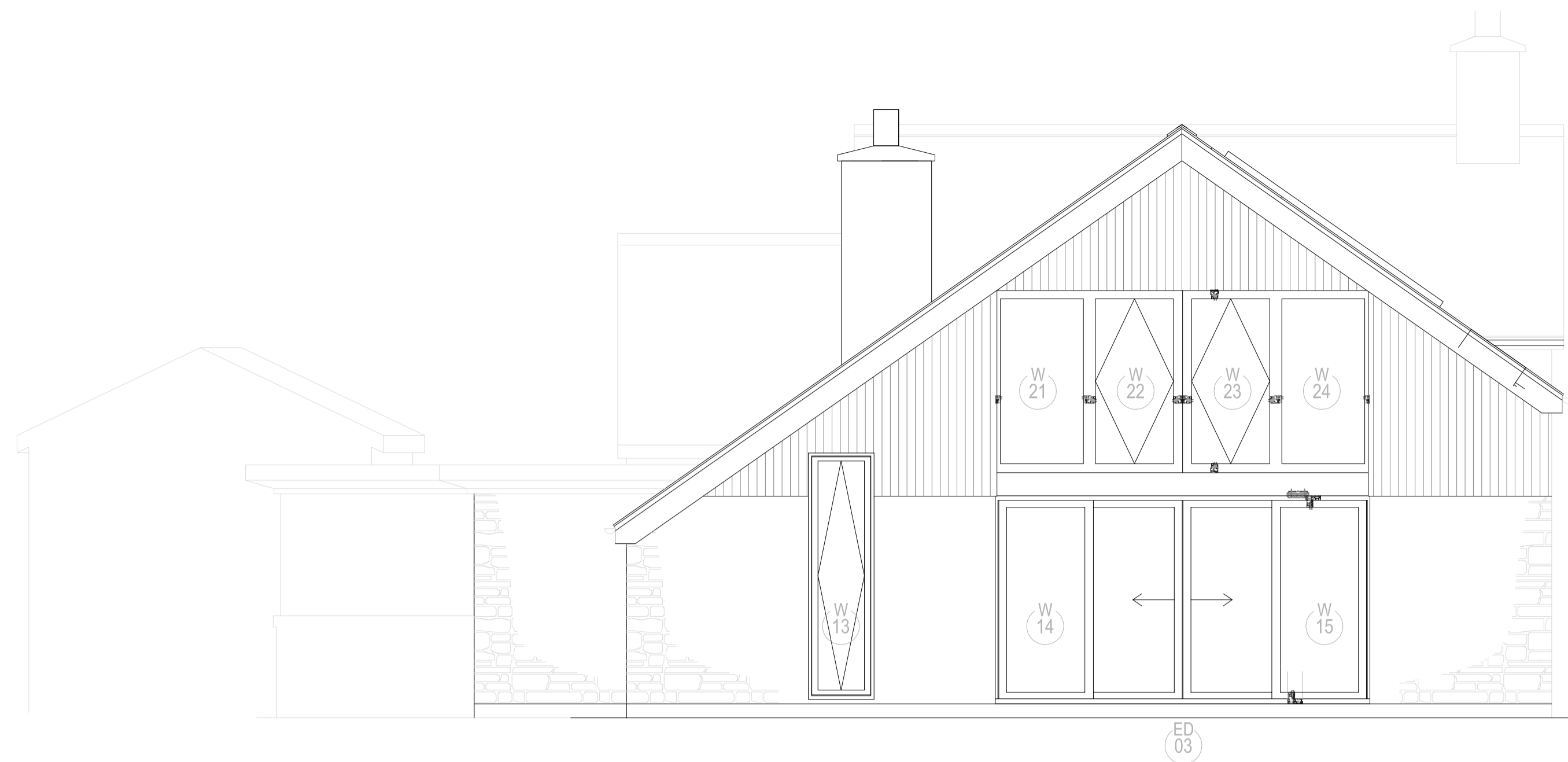
WEST ELEVATION 1:50
